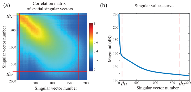
Fig. 1. Thresholds used for SVD filtering for patient 2, shown on (a) correlation pattern of spatial singular vectors (correlation matrix of spatial singular vectors) and (b) singular values' curve.
