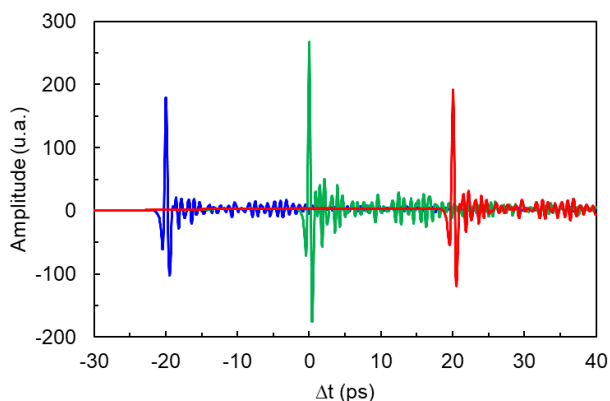
Figure 7: Respective quantitative impact on the delay and amplitude of the reflected THz pulse compared to the reference one (green).
