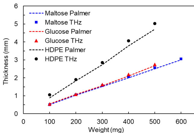
Figure 4: Comparison of samples thicknesses measured with palmer micrometer system (dashed lines) and evaluated using reflected THz pulses measurements (dots).
