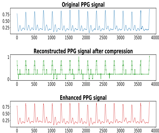
Fig. 9: Illustration of the enhancement of a compressed PPG batch using 1D-U-Net
