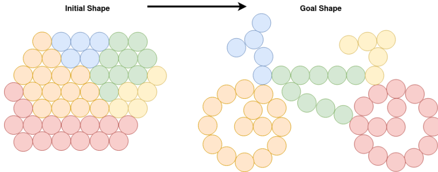
Fig. 2. Clustering motivation
