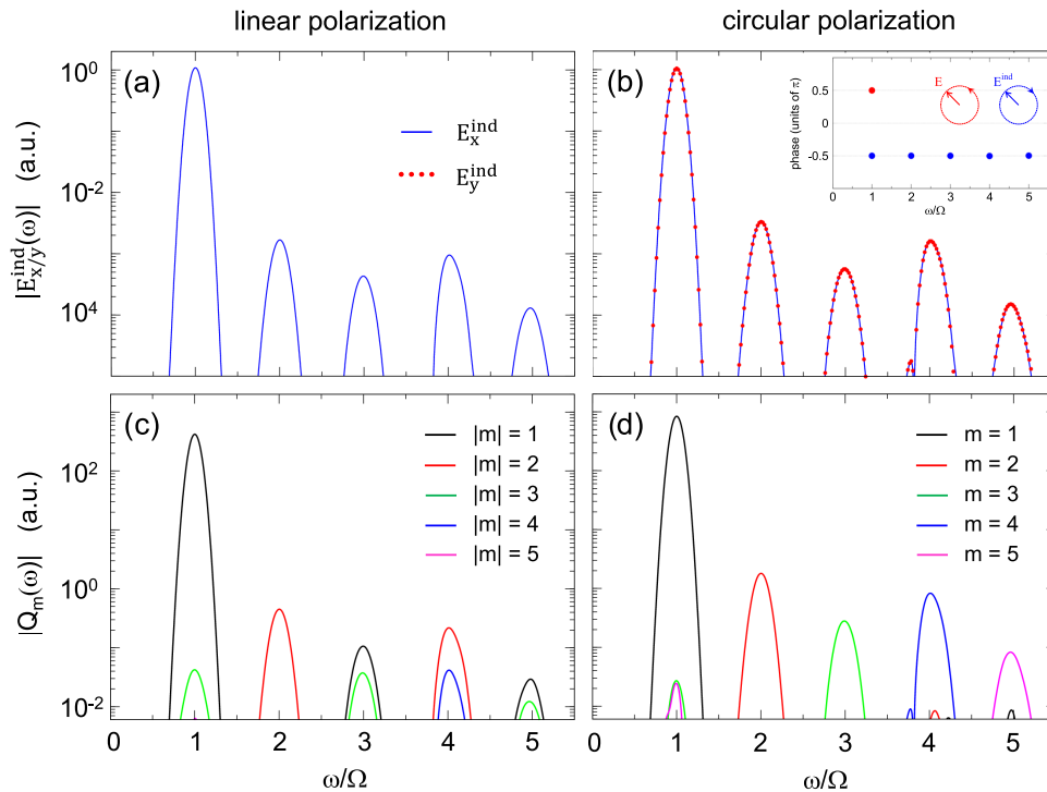
Figure 4. Spectral analysis of nonlinear near fields (a, b) and multipole moments (c, d) induced by the linearly (a, c) and circularly (b, d) polarized field with a fundamental frequency \Omega = 1.5 eV. Results are shown as a function of the frequency measured in units of the fundamental frequency \Omega . The TDDFT calculations are performed for an amplitude of the fundamental field E_0 = 5.2 \times 10^{-3} a.u. corresponding to an average power of the circularly polarized optical pulse of 2.4 \times 10^{12} W/cm 2 . (a, b) Frequency-resolved x - and y - components of the induced near field calculated at the x -axis at a distance d = 1.3 nm from the surface of the nanowire (see geometry in Figure 1). For the color code, see the inset of panel (a). The inset of panel b shows the phase between E_x and E_y components of the near field calculated at harmonic frequencies \omega = n\Omega (blue dots). The red dot indicates the corresponding phase for the fundamental field. (c, d) Frequency-resolved multipole moments |Q_m(\omega)| of the induced charge density. The color code corresponds to the multipole order m as explained in the insets. For the x -polarized fundamental field the results obtained for \pm m are degenerate. For a fundamental field with SAM = 1, the Q_m(\omega) are zero for nonpositive m \leq 0 .
