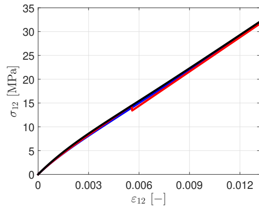
Figure 14. Comparison linear, bilinear and polynomial models: Evolution of the stress \sigma_{12} as a function of the strain \epsilon_{12} . Blue, red and black curves correspond to linear, bilinear and nonlinear cases, respectively.
