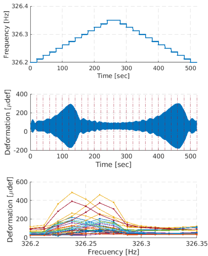
FIGURE 12: SOLUTION OF THE STEPPED-SINE TEST PERFORMED WITH \Delta\omega = 0.0125 HZ AND \Delta t = 20 S PER \omega . (TOP) EXCITATION PATTERN WITH TIME. (MIDDLE) TIME AMPLITUDE OF BLADE 1 DEFORMATION AT ROOT. (BOTTOM) FRF OF ALL BLADES ON 326.20 TO 326.35 HZ FREQUENCY RANGE.
