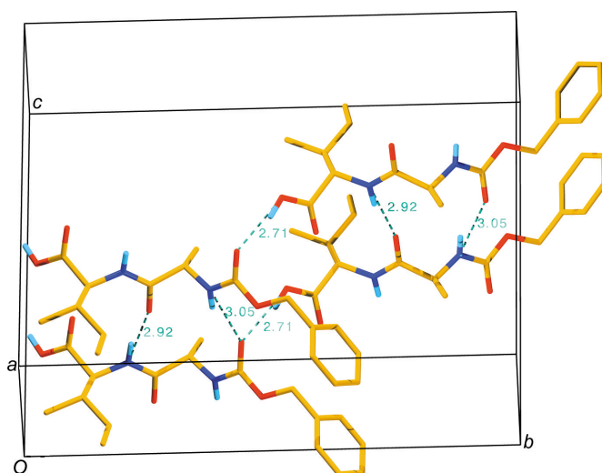
Figure 3 Hydrogen bonding of Z-Ala-Ile-OH, viewed approximately along the a axis. Hydrogen bonds are shown as dashed lines in cyan with the donor-acceptor distances ( D \cdots A ) in Å.
