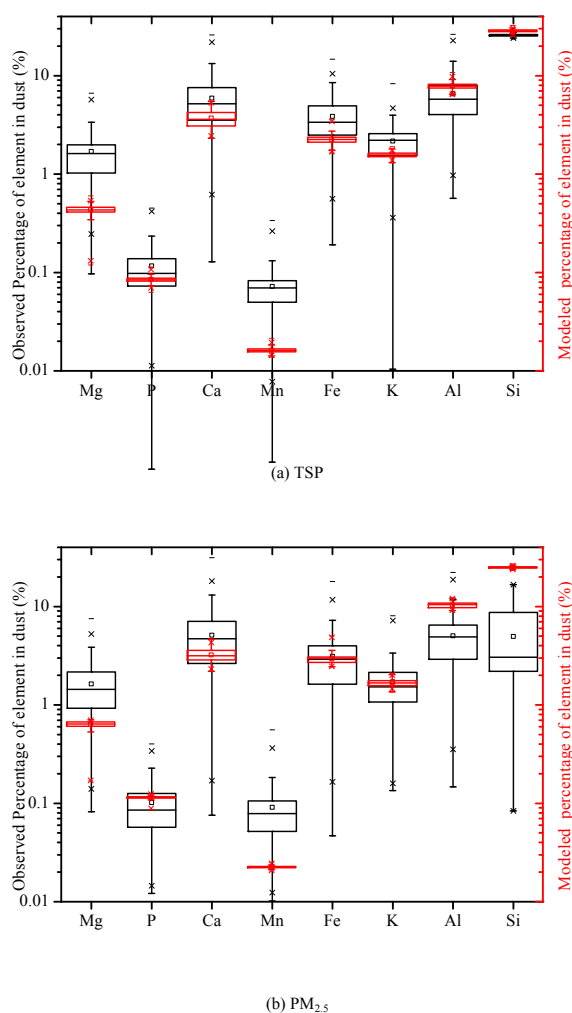
Figure 11. Mean and quartile modeled and observational fractions of elements in (a) TSP and (b) PM 2.5 for all sites together, the box line presents 25, 50 and 75 %, individually. Here we calculate the elemental fractions and average the fractions temporally for each site and compare to observations.
