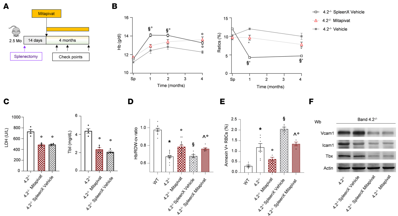
Figure 6. Noninferiority of mitapivat versus splenectomy in 4.2^{-/-} mice is associated with protection against hemolysis-induced inflammatory vasculopathy. (A) Experimental design to study the effect of splenectomy in combination with mitapivat (100 mg/kg/d) in 4.2^{-/-} mice. (B) Hb levels and reticulocyte count in 4.2^{-/-} mice treated with vehicle or mitapivat (100 mg/kg/d) or splenectomized (splenx) monitored up to 7 months of age. Data are reported as mean \pm SEM; 4.2^{-/-} vehicle, n = 5-7 ; 4.2^{-/-} mitapivat, n = 5-7 ; 4.2^{-/-} splenx, n = 6 . ^{\circ}P < 0.05 compared with vehicle-treated 4.2^{-/-} mice; ^{\$}P < 0.05 compared with mitapivat-treated 4.2^{-/-} mice (1-way ANOVA with Dunnett's longitudinal comparison). (C) Plasma LDH and total bilirubin (Tbil) levels in 4.2^{-/-} mice treated as described in A. Data are reported as mean \pm SEM ( n = 4 ); ^{\circ}P < 0.05 compared with vehicle-treated 4.2^{-/-} mice (1-way ANOVA). (D and E) Hb to RDW ratio and annexin-V + RBCs from WT and 4.2^{-/-} mice with or without spleen and treated with either vehicle or mitapivat (100 mg/kg/d). Data are reported as mean \pm SEM ( n = 4-15 ). ^*P < 0.05 compared with WT mice, ^{\circ}P < 0.05 compared with vehicle-treated 4.2^{-/-} mice (1-way ANOVA). (D and E) ^{\$}P < 0.05 compared with mitapivat-treated 4.2^{-/-} mice; ^{\wedge}P < 0.05 compared with splenx 4.2^{-/-} mice treated with vehicle (2-way ANOVA). (F) IB analysis using specific Abs against Vcam1, Icam1, and Tbx in isolated aortas from 4.2^{-/-} mice with or without spleen and treated with either vehicle or mitapivat. Protein (50 \mu\text{g}/\mu\text{L} ) loaded on an 8% T, 2.5%C polyacrylamide gel. Actin was the protein loading control. One representative gel from 3-5 with similar results is shown. Densitometric analysis of IBs is shown in Supplemental Figure 9B. Wb, Western blot.
