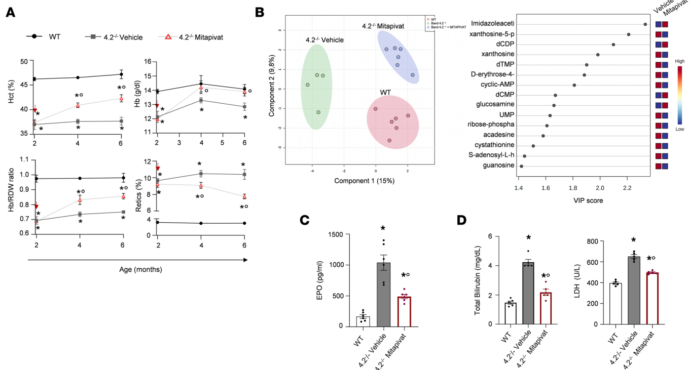
Figure 2. Mitapivat improves anemia by metabolic reprogramming of 4.2 -/- mouse RBCs. (A) Hct, Hb, and Hb to RDW ratio, as marker of spherocytosis and reticulocyte count in WT and 4.2 -/- mice treated with vehicle or mitapivat (100 mg/kg/d) up to 6 months of age. The red arrow indicates the starting point for mitapivat administration. Data are reported as mean ± SEM (WT, n = 5; 4.2 -/- vehicle, n = 9; 4.2 -/- mitapivat, n = 12). *P < 0.05 compared with WT; °P < 0.05 compared with vehicle-treated 4.2 -/- mice by 1 way ANOVA with Dunnett's longitudinal comparison. (B) 2D PCA scores obtained from the analysis of untargeted metabolites of RBCs from WT and 4.2 -/- mice treated with vehicle or mitapivat (100 mg/kg/d) for 6 months. The value of each biological replicate was normalized. Data on WT animals are in red, on 4.2 -/- mice are in green, and on mitapivat-treated 4.2 -/- mice are in blue (n = 4–6). The variable importance in projection (VIP) score plot for the top 15 most important metabolite features identified by partial least squares discriminant analysis (PLS-DA). The box indicates the relative concentration from vehicle and mitapivat groups (right panel). Figures were created using MetaboAnalyst 5.0. (C and D) Plasma EPO, total bilirubin, and LDH, as markers of hemolysis, in WT and 4.2 -/- mice treated with vehicle or mitapivat (100 mg/kg/d) for 6 months (n = 5). *P < 0.05 compared with WT; °P < 0.05 compared with vehicle-treated 4.2 -/- mice by 1-way ANOVA. dCMP, deoxycytidine monophosphate; dTMP, deoxytimidine monophosphate; AMP, adenosine monophosphate; UMP, uridine 5-monophosphate.
