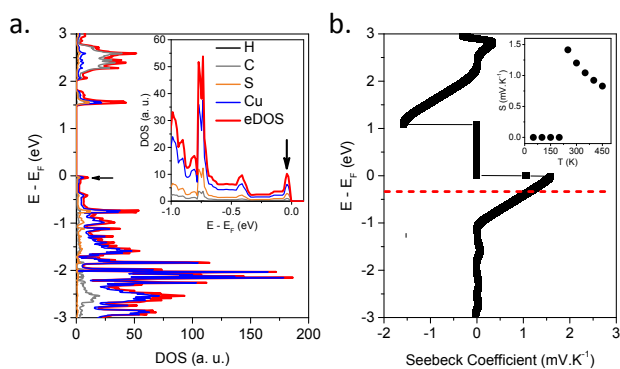
Figure 3. a. Calculated density of states (DOS) of [\text{Cu}_2(1,3\text{-BDT})]_n : projected electronic DOS (p-eDOS) with grey line for C, black for H, orange for S and blue for Cu electrons and the total electronic DOS (eDOS) in red. The insert is a zoom close to the Fermi level and with switched axes. The black arrows show the sharp peaks associated to high Seebeck coefficient. b. Calculated Seebeck coefficient at 300 K. The insert shows its temperature dependence at constant energy represented by the dotted red line on the Figure b.
