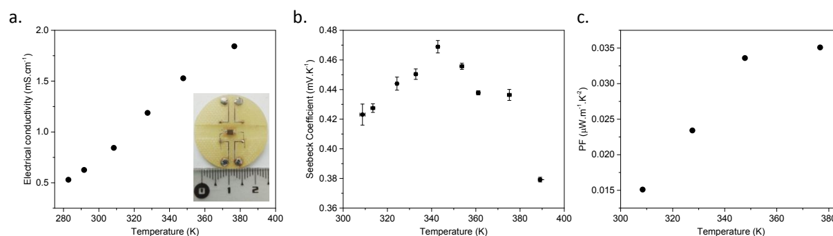
Figure 2. a. Temperature dependence of the electrical conductivity measured on a [\text{Cu}_2(1,3\text{-BDT})]_n pressed pellet by surface four-probe configuration and photo of the device to apply the bulk measurement of the electrical conductivity; b. Seebeck coefficient with temperature (errors come from the linear fits of the raw data) and c. the power factor with temperature.
