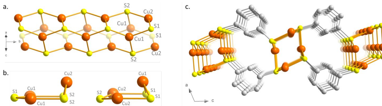
Figure 1. Structure of [\text{Cu}_2(1,3\text{-BDT})]_n : a. the Cu-S chain along the b axis; b. the two deformed \text{Cu}_3\text{S}_3 hexagons and c. the central projection along the b axis. Orange, yellow and gray spheres correspond to copper, sulfur and carbon atoms. Hydrogen atoms were omitted for clarity.
