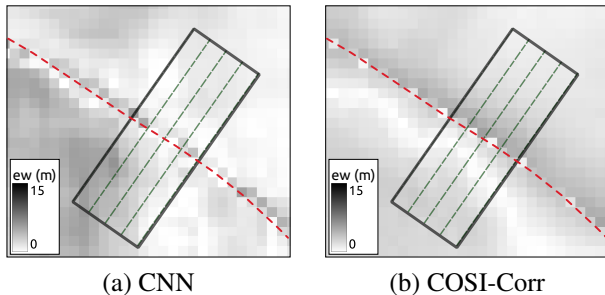
Fig. 3. East-West close ups of residual maps (absolute displacement error), in meters. Red line shows the discontinuity trace. Dark green dashed lines show fault-perpendicular profile locations from Figure 4.
