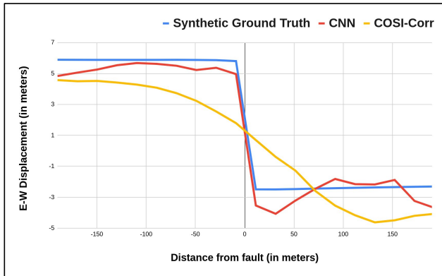
Fig. 4. Profile across fault of the synthetic ground truth, CNN and COSI-Corr correlation maps. This profile is computed by averaging three neighbouring profiles. See Figure 3 for profile locations.
