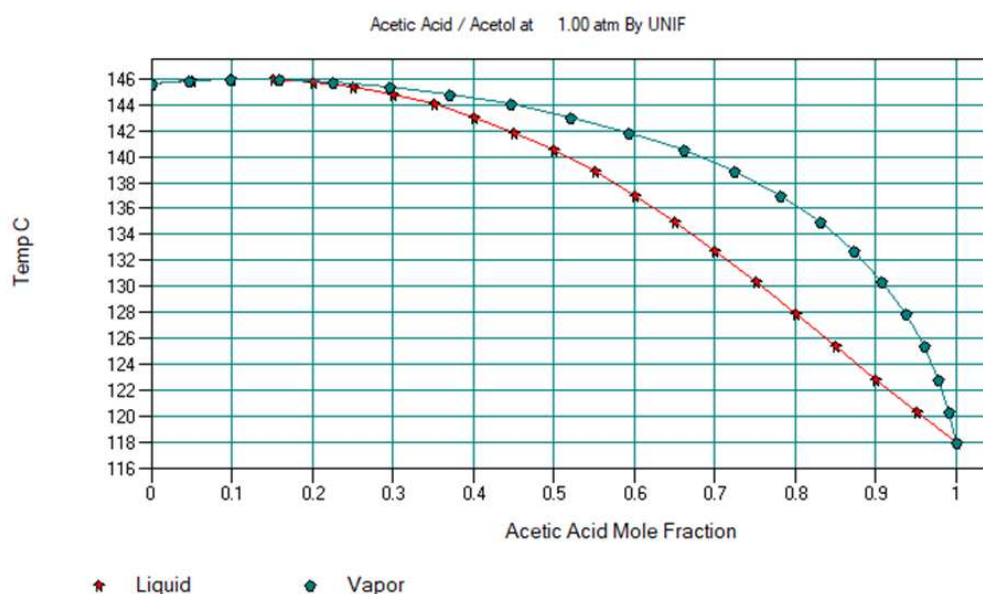
Figure 1. Equilibrium data for the A/HAc system.
