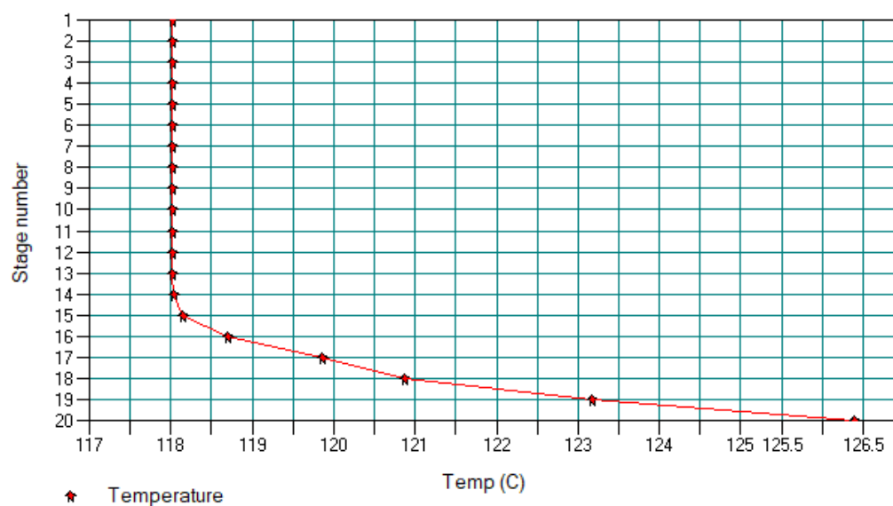
Figure 8. Tray temperature profile in column 2.
