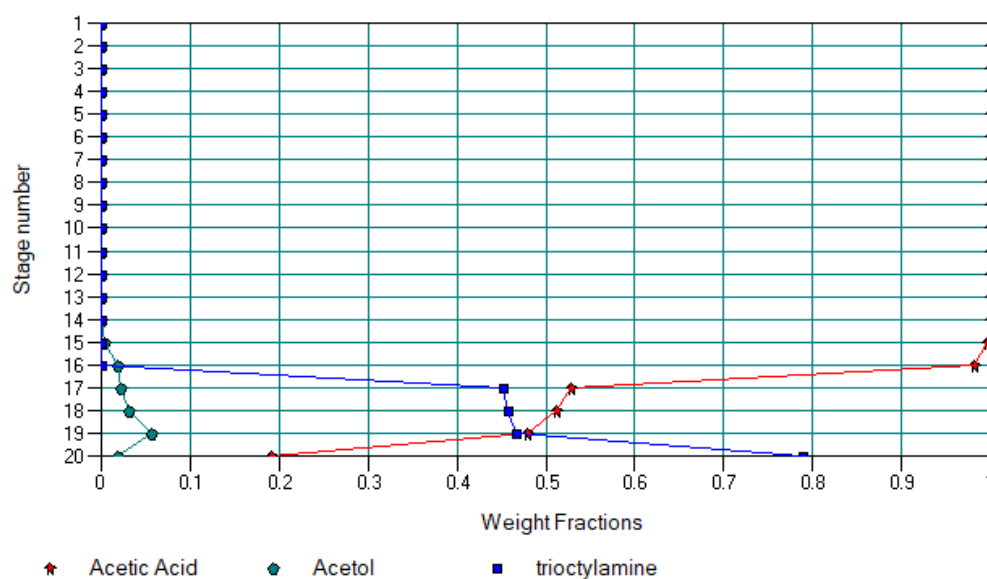
Figure 7. Tray liquid concentration profile in column 2.
