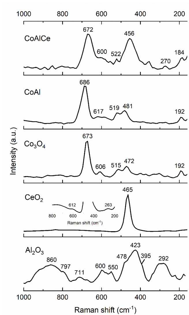
Figure 4. Raman spectra of the mixed and single oxides.
