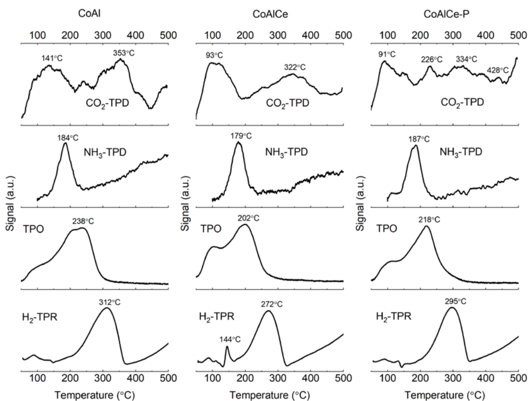
Figure 5. Temperature-programmed reduction, oxidation, NH 3 desorption and CO 2 desorption profiles for the CoAl, CoAlCe and CoAlCe-P samples.
