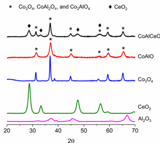
Figure 3. XRD diffractograms of calcined CoAl, CoAlCe, \text{Co}_3\text{O}_4 , \text{CeO}_2 and \text{Al}_2\text{O}_3 .
