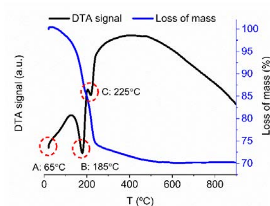
Figure 1. TGA-DTA results of the CoAl hydrotalcite precursor.
