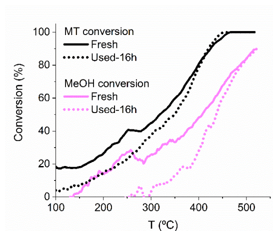
Figure 10. Methanethiol and methanol conversion vs. temperature before (fresh) and after (16 h) the stability test with the CoAlCe-P catalyst.
