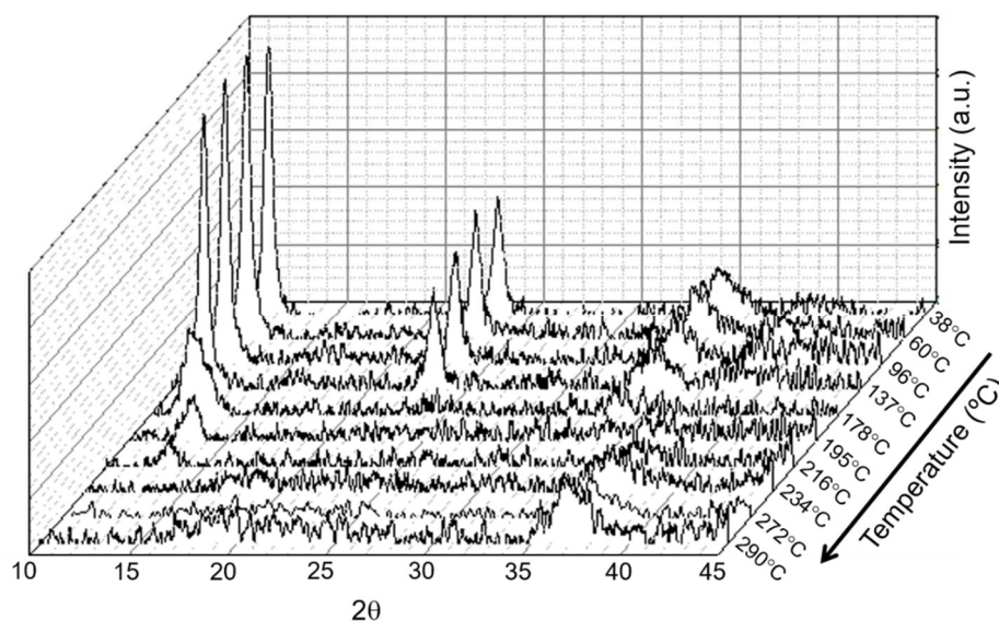
Figure 2. Temperature-programmed XRD diffractograms of CoAl starting from hydrotalcite and ending up to a mixed metal oxide structure.
