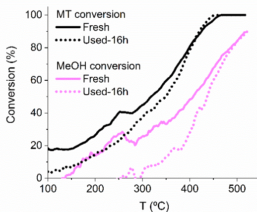
Figure 10. Methanethiol and methanol conversion vs. temperature before (fresh) and after (16 h) the stability test with the CoAlCe-P catalyst.
