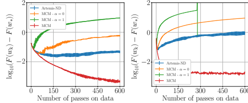
Figure 1: Comparing MCM on two datasets with three other algorithms using a non-degraded update, \gamma = 1/L . Artemis-ND stands for Artemis with a non-degraded update.
