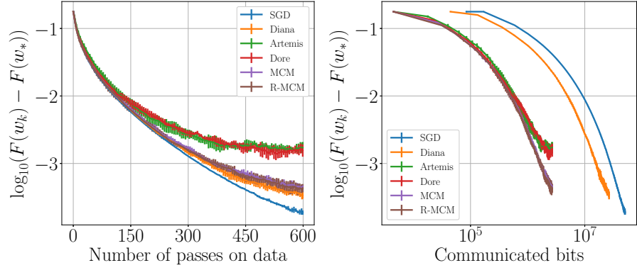
(a) X axis in # iterations. (b) X axis in # bits. Figure S3: quantum with b = 400 , \gamma = 1/L .
