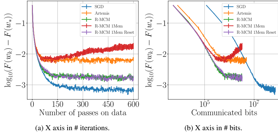
Figure S10: A9A with b = 50 , \gamma = 1/L and a 2-quantization. Only half of the devices are participating at each round.
