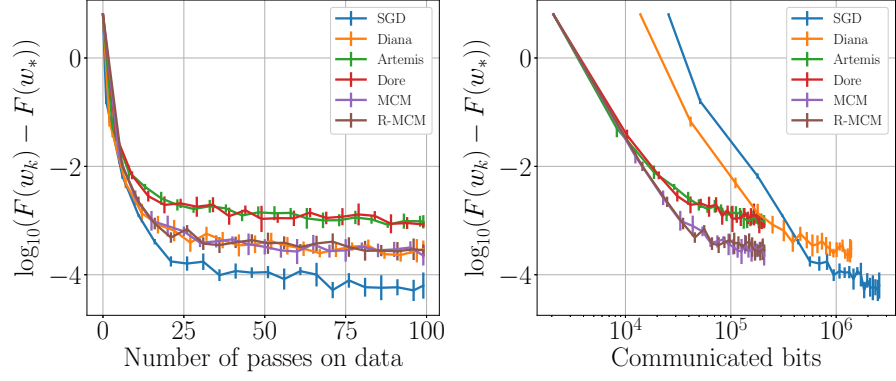
(a) X axis in # iterations. (b) X axis in # bits. Figure S1: Least-square regression, toy dataset: \gamma = (L\sqrt{k})^{-1} , \sigma \neq 0 .
