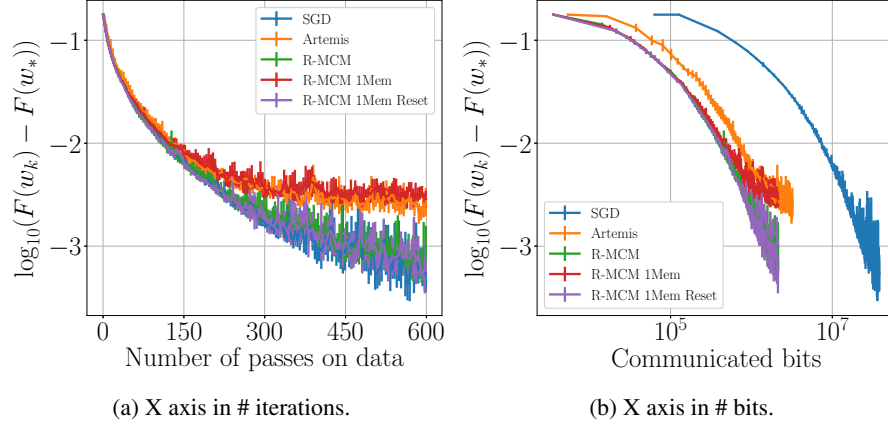
Figure S9: quantum with b = 400 , \gamma = 1/L and a 2-quantization. Only half of the devices are participating at each round.
