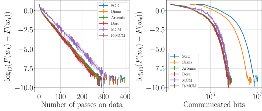
(a) X axis in # iterations. (b) X axis in # bits. Figure S2: Least-square regression, toy dataset: \gamma = 1/L , \sigma_*^2 = 0 .
