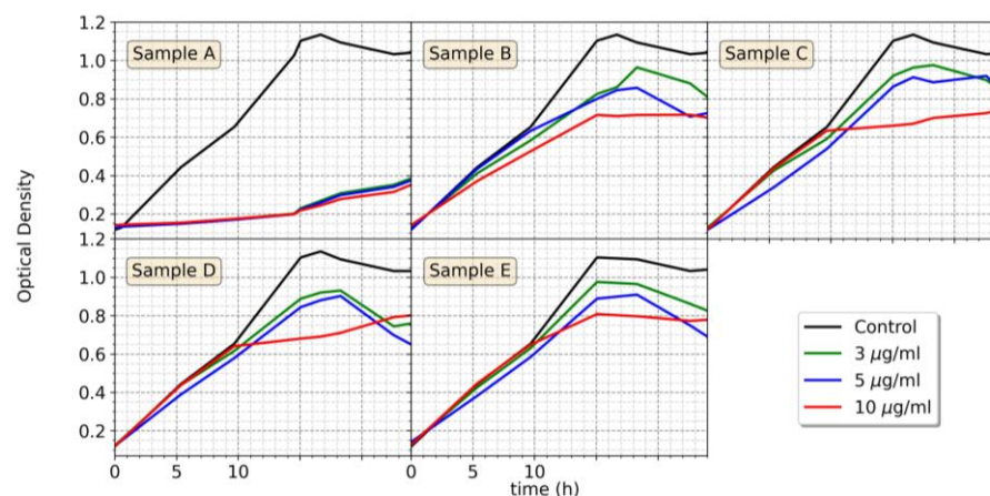
Figure 8. Growth curve of E. coli under aerobic conditions in the absence or presence of AgNPs (samples A–E) with concentrations ranging from 3 to 10 \mu\text{g/mL} .
