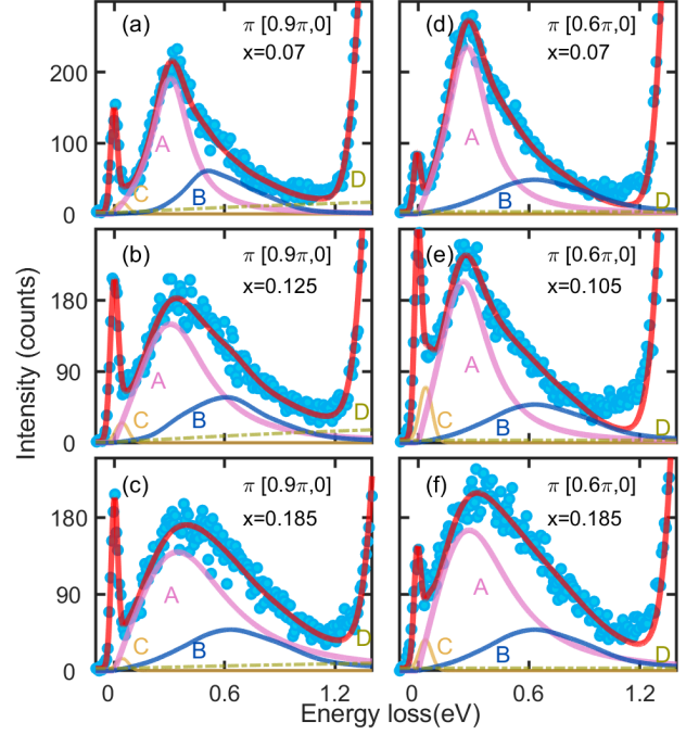
FIG. 2: Results from cross-fitting approach. (a)-(c): \mathbf{Q}_{\parallel} = [0.9\pi, 0] ; (d)-(f) \mathbf{Q}_{\parallel} = [0.6\pi, 0] . The overall spectra are decomposed into elastic peak, paramagnon A , multimagnon B , phonon C , and a small linear background D . Dots are the experimental data points.
