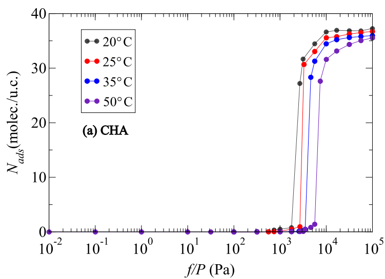
(a) Chabazite
