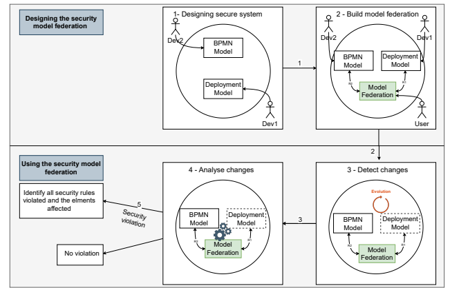
Fig. 1. Excerpt of the security-oriented model federation methodology
