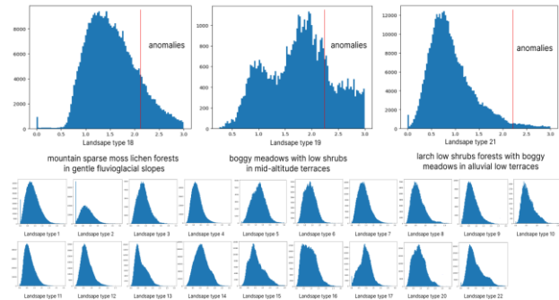
Figure 3. Histograms of standard deviation LST values by types of permafrost landscapes with detection of thermal anomalies
