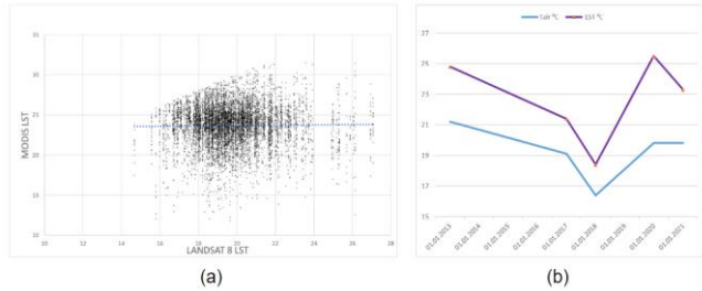
Figure 1. (a) Linear regression of LST MODIS with LST obtained by Landsat 8 in the study area (b) Comparison of LST obtained by Landsat 8 with air temperature from a weather station
