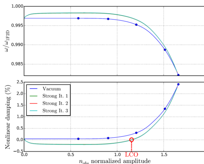
FIGURE 9: APPLICATION OF THE STRONG COUPLING PROCEDURE ON DP20 OPERATING POINT. ● : EXTRACTION POINTS FROM THE NONLINEAR DYNAMICS IN VACUUM
