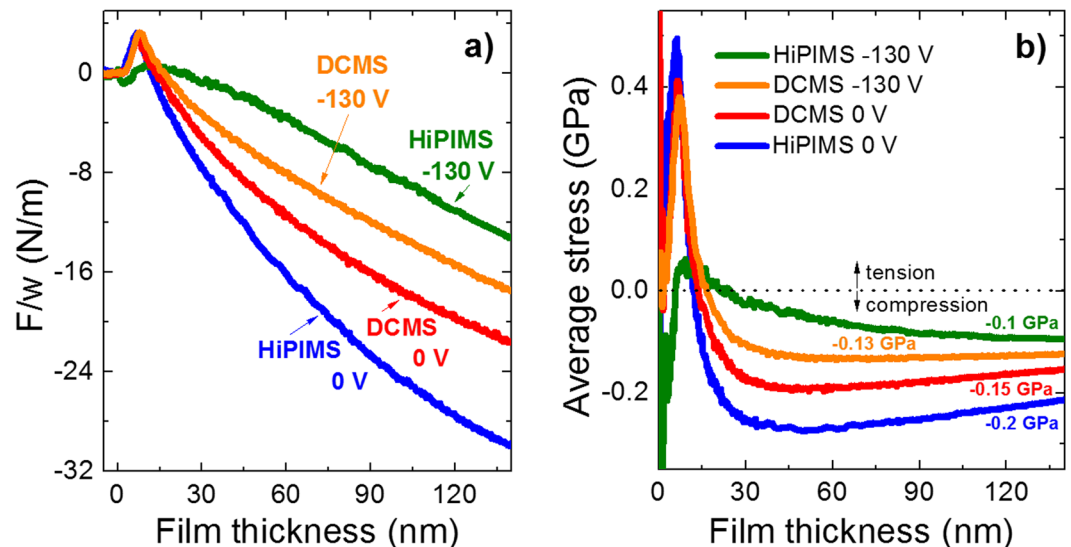
Figure 3. In situ intrinsic stress measurements during thin film growth. Evolution of (a) the film force per unit width, F/w , and (b) average stress, \langle \sigma \rangle , as a function of film thickness for grounded (0 V) and -130 V bias DCMS and HiPIMS Cu films.
