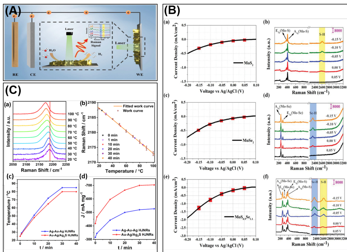
Figure 16. (A) The schematic of the photoelectrochemical system with LSV-Raman analysis. The measured material is \text{MoS}_{2\text{x}}\text{Se}_{2(1-x)} . The reference electrode, counter electrode, and working electrode are termed as RE, CE, and WE, respectively. Evolution of (B) LSV vs. the voltage (0.05, 0.00, -0.05, -0.10, and -0.15 V) and the Raman spectra of the samples (a,b) \text{MoS}_2 , (c,d) \text{MoSe}_2 and (e,f) \text{MoS}_{0.9}\text{Se}_{1.1} . (C) (a) SERS spectra of MI on the Au–Ag/Ag 2 S HJNRs at different temperatures. (b) Dependence of fitted temperature on the Raman shifts of MI for the Au–Ag/Ag 2 S HJNRs. (c) Hot spots temperatures of the Ag–Au–Ag and Au–Ag/Ag 2 S HJNRs illuminated for different times; (d) photocatalytic activity of the Ag–Au–Ag and Au–Ag/Ag 2 S HJNRs illuminated for different times. (Copyright with permission from Ref. [92,93]).
