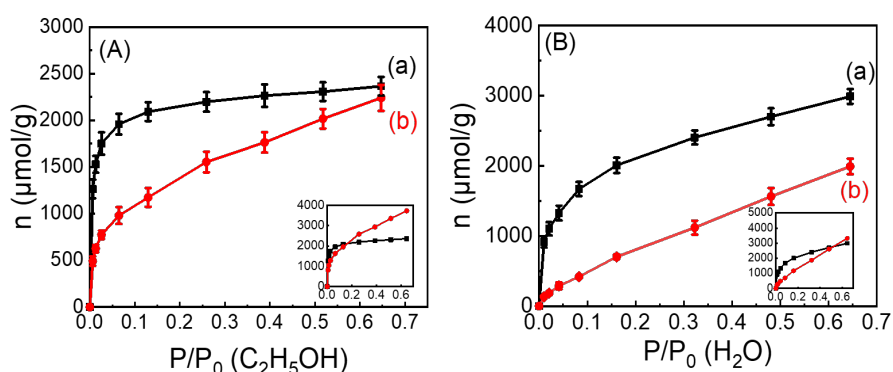
Figure 8: (A) Ethanol and (B) water gravimetric adsorption isotherms on MFI ((a)- black) and MFI@Polymer ((b)- red). The adsorptions were conducted at RT. The insets figures correspond to the adsorbed quantities of ethanol and water after normalization to the mass of zeolite, determined from the TG (60 % of zeolites in the sample MFI@Polymer).
