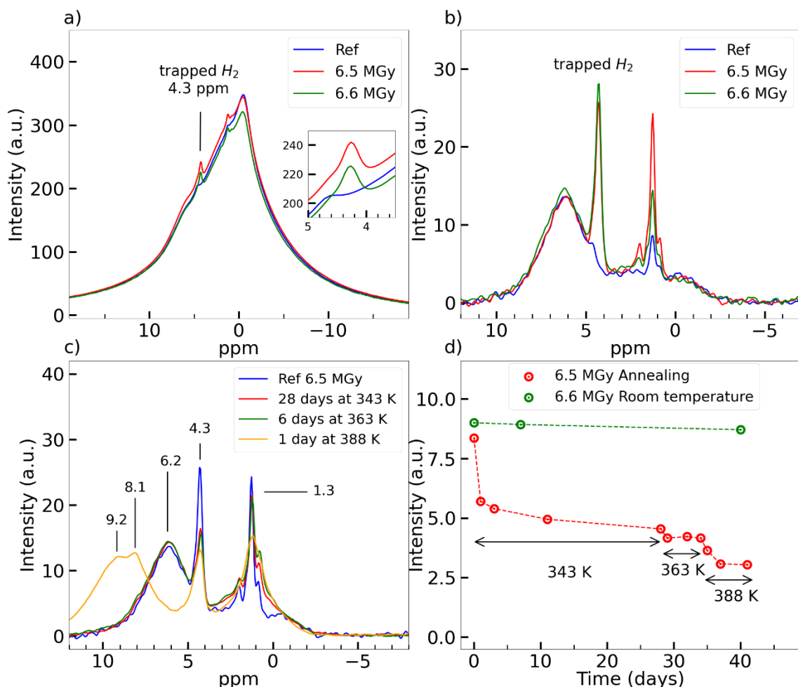
Figure 8. ^1\text{H} MAS NMR analysis of portlandite. a, b) Comparison of NMR spectra of irradiated (red & green) and non-irradiated portlandite (blue); a) echo time of 80\ \mu\text{s} ; b) echo time of 2 ms. c) Influence of successive annealing treatments on the NMR spectrum of portlandite irradiated at 6.5 MGy. The spectra were recorded with an echo time of 2 ms. d) Time evolution of the intensity of the 4.3 ppm peak associated to trapped \text{H}_2 at room temperature (in green), and with successive annealing temperatures (in red).
