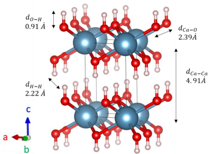
Figure 1. Structure of Ca(OH) 2 and interatomic distances. Figure realized on Vesta 18
