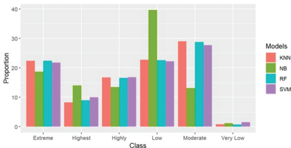
Figure 14. Relative proportions of vulnerability classes by machine learning model.
