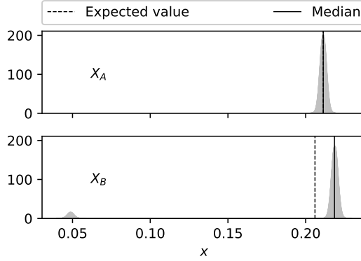
Figure 4: Case 2. The probability density functions of X_A and X_B : g_A = g_{\mathcal{N}(0.211325, 0.002)} and g_B = 0.925 \cdot g_{\mathcal{N}(0.21875, 0.002)} + 0.075 \cdot g_{\mathcal{N}(0.04875, 0.002)} respectively.
