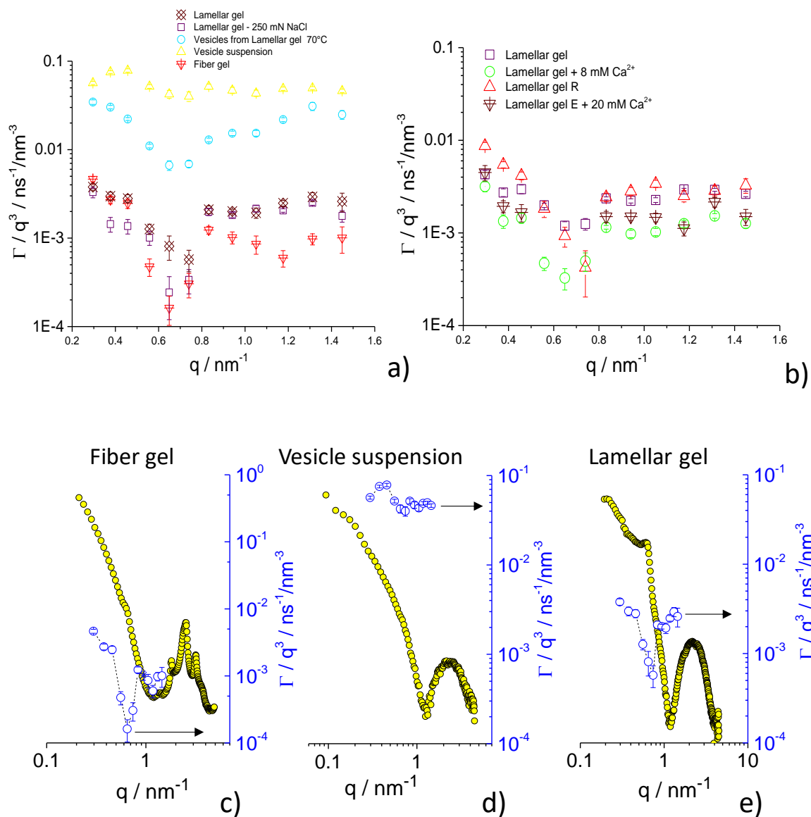
Figure S 2 – a-b) Evolution of the Zilman-Granek decay parameter as a function of the full-range wavevector, q , for various G-C18:1 (Vesicles suspension, Fiber gel) and G-C18:0 (Lamellar gel) self-assembled samples. Sample labelled “Vesicles from Lamellar Gel @ 70°C” corresponds to “Lamellar Gel – 250 mM NaCl” heated at 70°C. The “R” in b) stands for “Replicate” and it refers to a freshly-made new sample.
