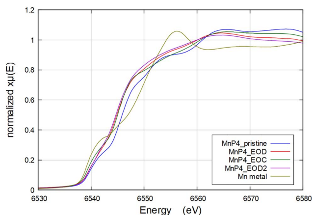
Fig. 10 Mn K-edge XANES spectra of \text{MnP}_4 electrodes containing 74 wt% of active material in the pristine state (blue), stopped at 0 V at the end of the first discharge (red), at the end of the first charge (green) and at the end of the second discharge (violet).
