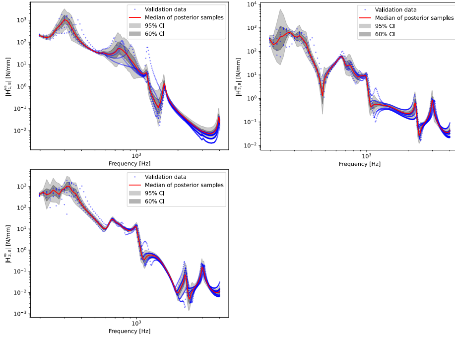
Figure 14: Magnitude of posterior predicted samples of the transfer function \mathbf{H}_{d,k}^{\text{MB}} from the left mount to the vehicle body in all three directions for the mechanical order k = 8
