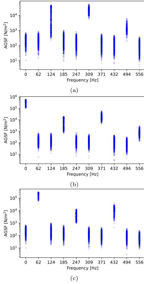
Figure 5: Air-gap surface force [N/m 2 ] samples generated for different spatial orders at \Omega = 463 RPM for three different spatial orders (a) shows AGSF for r = -8 , (b) for r = 0 and (c) for r = +8
