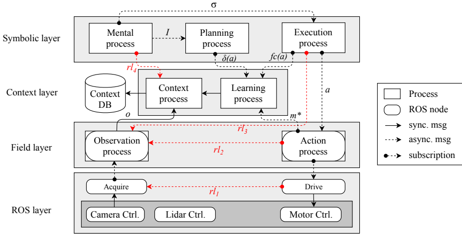
Figure 1. Embedded Higher-order Agent (E-HoA) architecture
