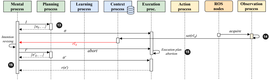
Figure 6. Functioning of intent-reflex ( rl_4 ) strategy
