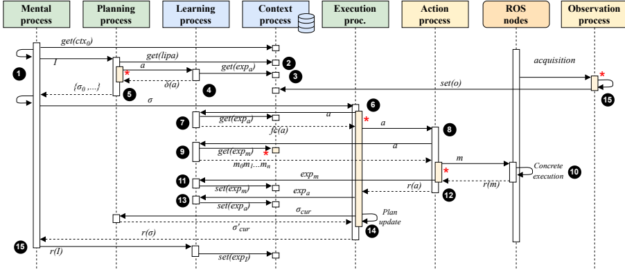
Figure 2. Nominal E-HoA execution loop
