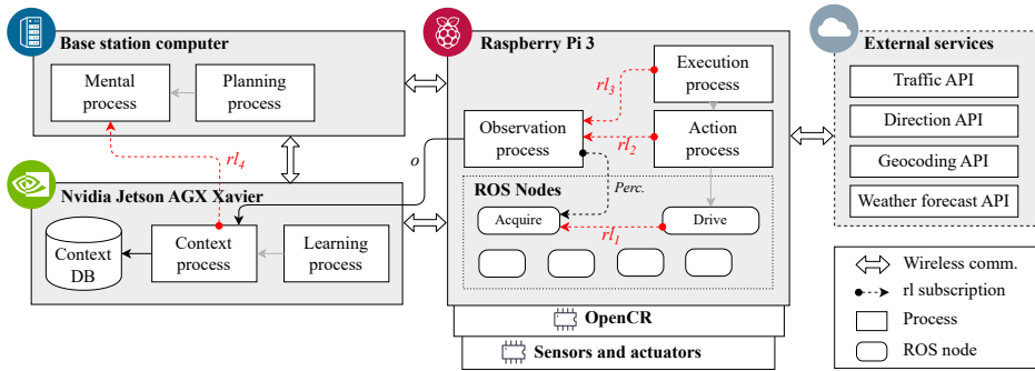
Figure 8. A possible hardware deployment for E-HoA architecture
