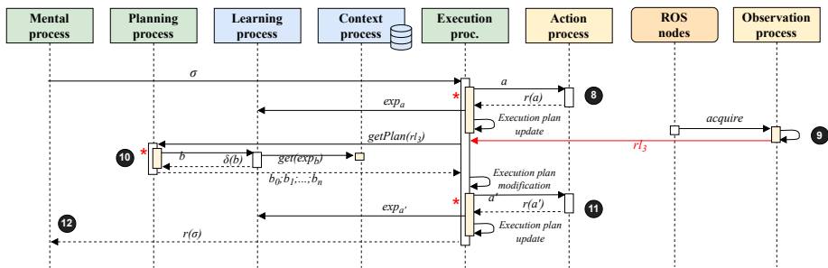
Figure 5. Functioning of action-reflex ( rl_3 ) strategy
