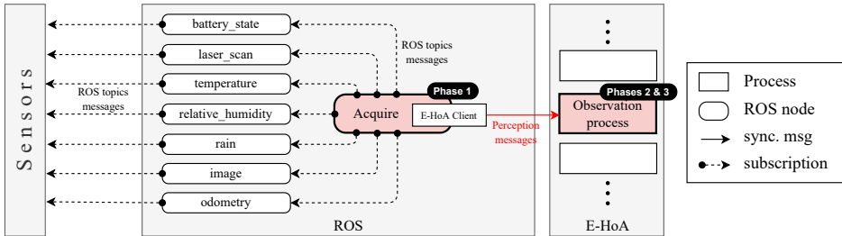
Figure 7. Observation System Architecture
