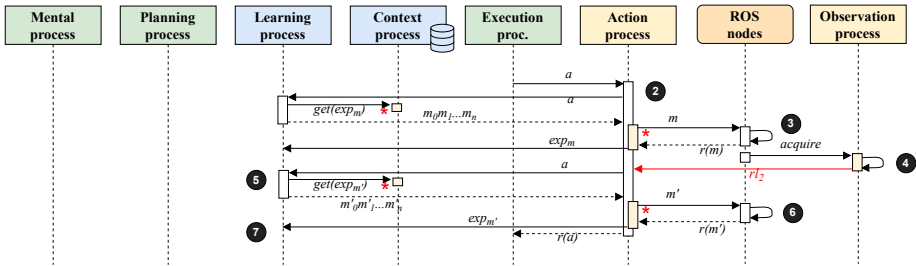
Figure 4. Functioning of field-reflex ( rl_2 ) strategy
