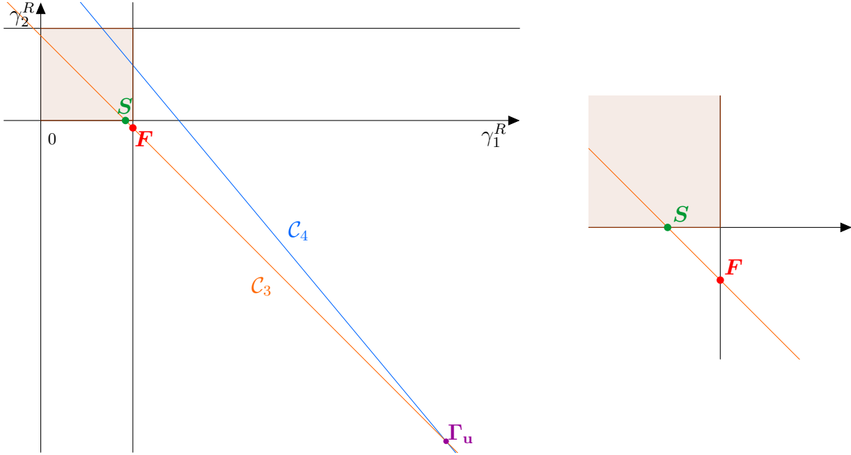
Figure 11: Graphical resolution of the 2 \times 2 LP problem. Polytope of the constraints (left) and a zoom (right). F is the erroneous solution and S is the correct one.
