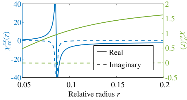
Fig. 9. Surface susceptibilities associated with the circular meta-atoms of section 3.1 obtained by solving the elementary problems of eq. (16) for different radius.
