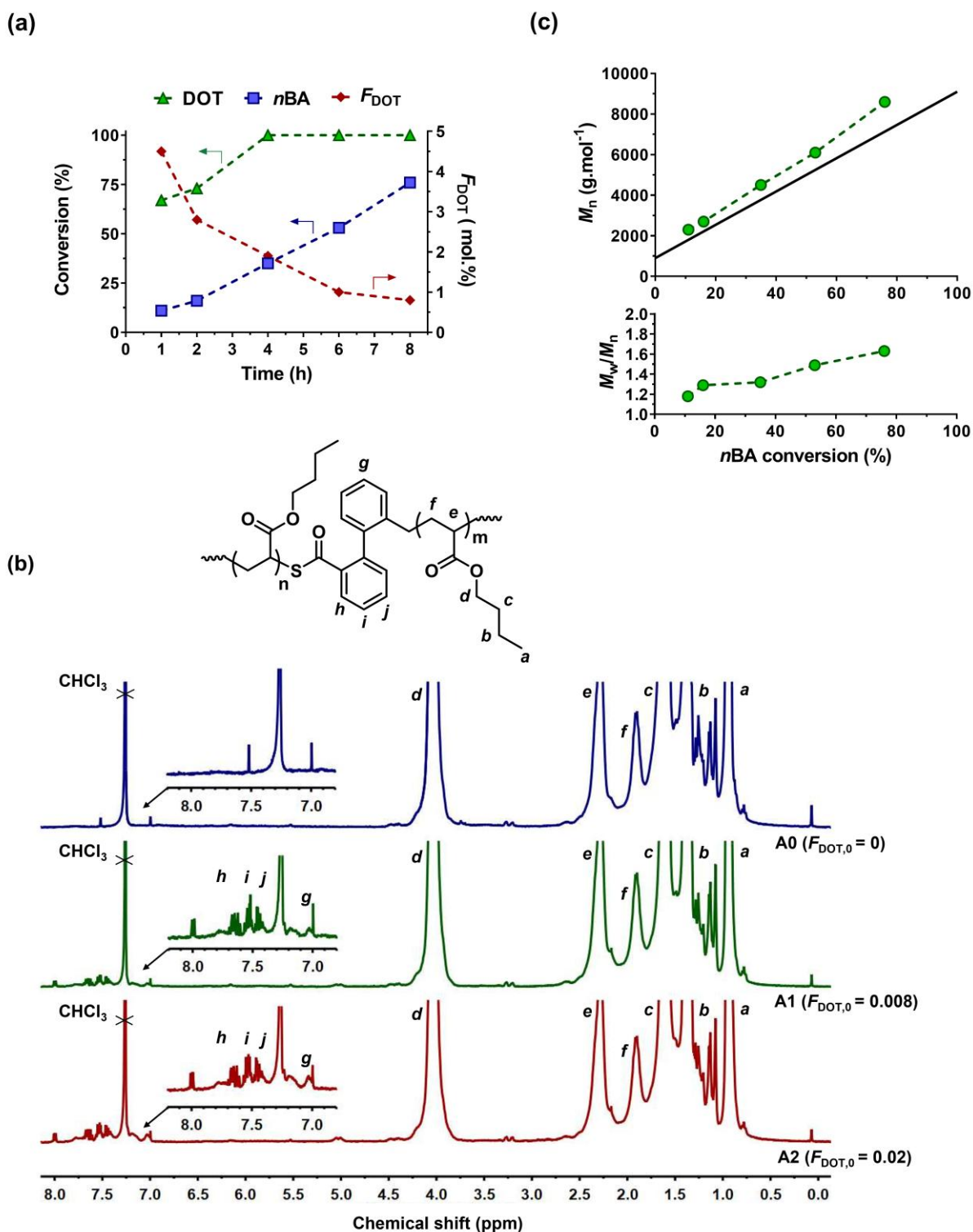
Figure 3. Synthesis of PnBA-b-P(nBA-co-DOT) copolymer latexes by copolymerization of nBA and DOT in water at 110\text{ }^{\circ}\text{C} initiated by PnBA -SG1 seeds ( A1 , Table 1): (a) evolution of nBA conversion, DOT conversion and average molar fraction of DOT ( F_{DOT} ) in the whole copolymer vs. time; (b) ^1\text{H} NMR spectra (400 MHz, \text{CDCl}_3 ) in the 0–8 ppm region of PnBA - b - P(nBA-co-DOT) copolymers A0 , A1 and A2 ; (c) evolution of M_n and \bar{D} vs. nBA conversion ( A1 ).
