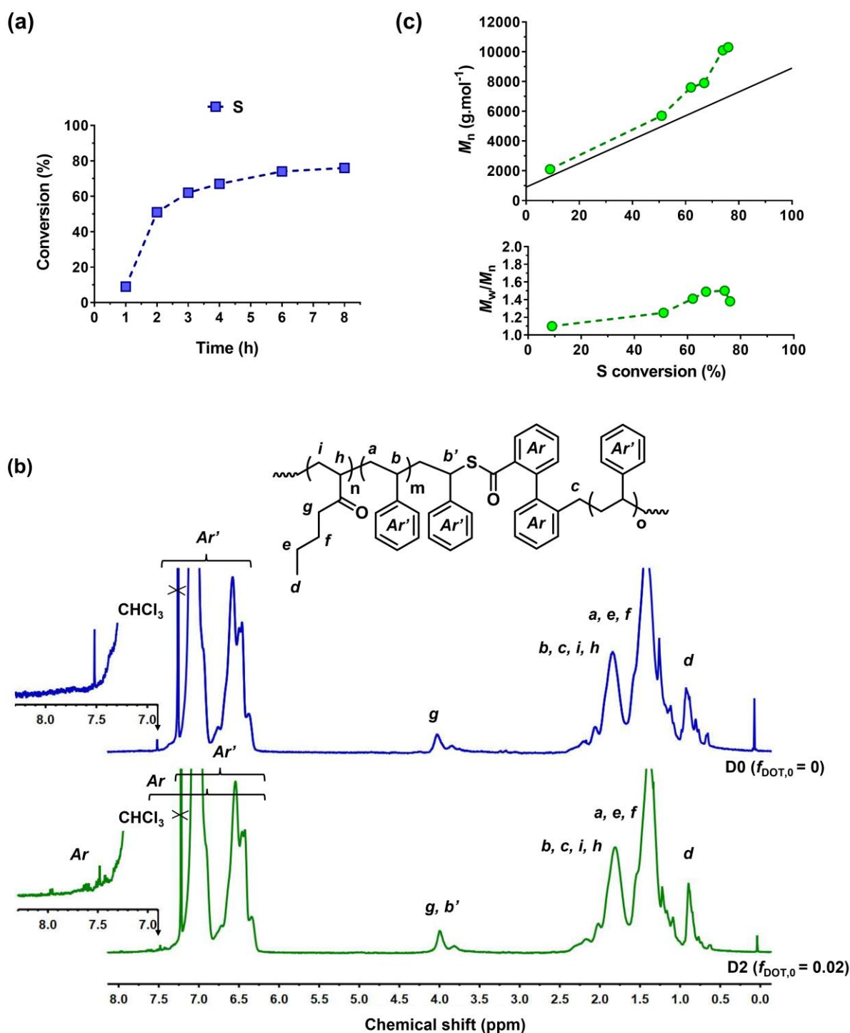
Figure 5. Synthesis of PnBA- b -P(S-co-DOT) copolymer latexes by copolymerization of S and DOT in water at 110 °C initiated by PnBA-SG1 seeds ( D2 , Table 1): (a) evolution of S conversion in the copolymer vs. time (DOT conversion could not be determined due to the overlapping protons (peak g ) of n BA and the overlapping aromatic protons (peaks Ar') of S, with those of DOT); (b) 1 H NMR spectra (400 MHz, CDCl 3 ) in the 0–8 ppm region of PnBA- b -P(S-co-DOT) copolymers D0 and D2 and (c) evolution of M_n and \bar{D} vs. S conversion.
