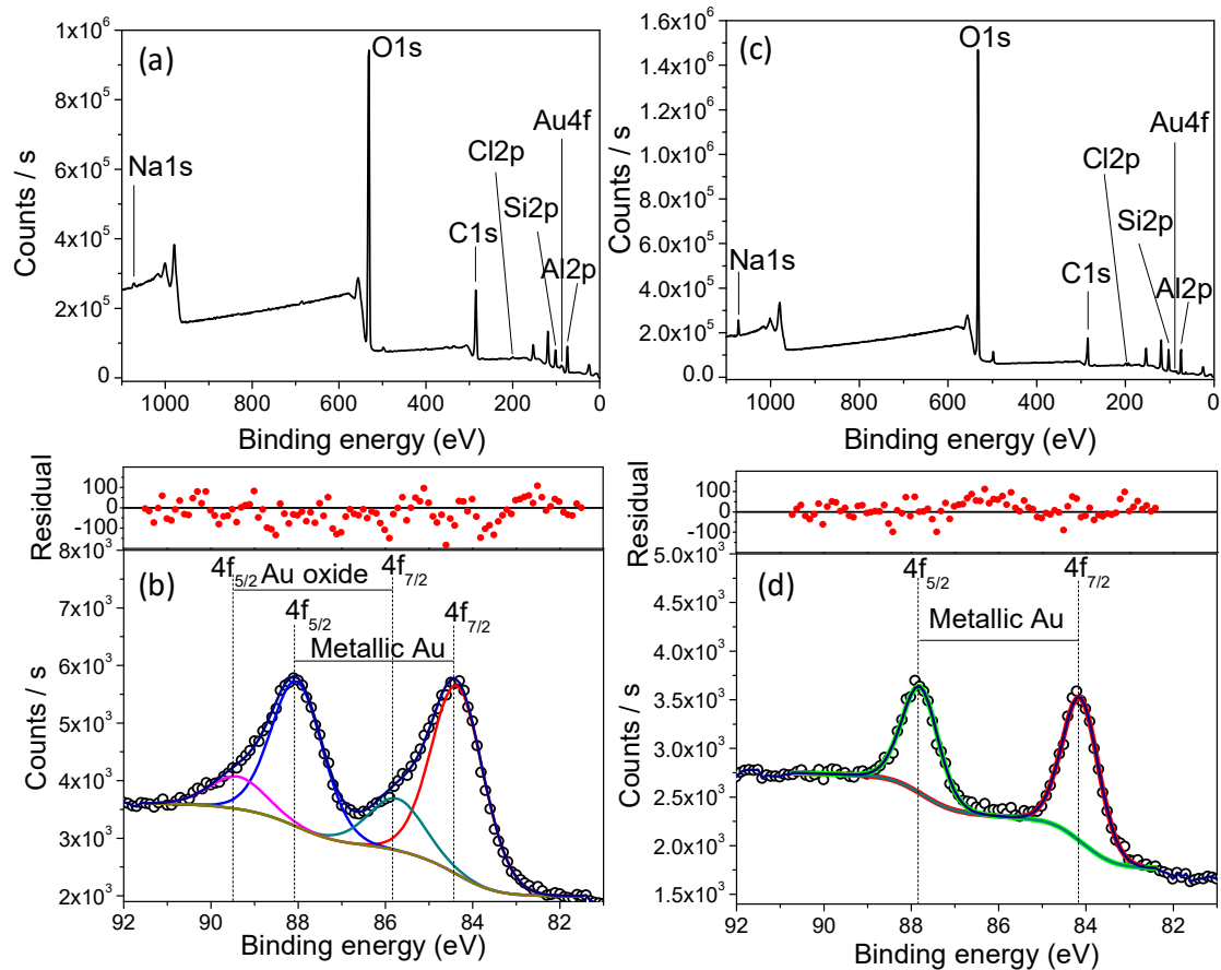
Figure 4. XPS survey and Au 4f photoelectron core-level spectra of GNPs attached to Imo-CH 3 NTs prepared by UV photolysis (a,b) and gamma radiolysis (c,d).
