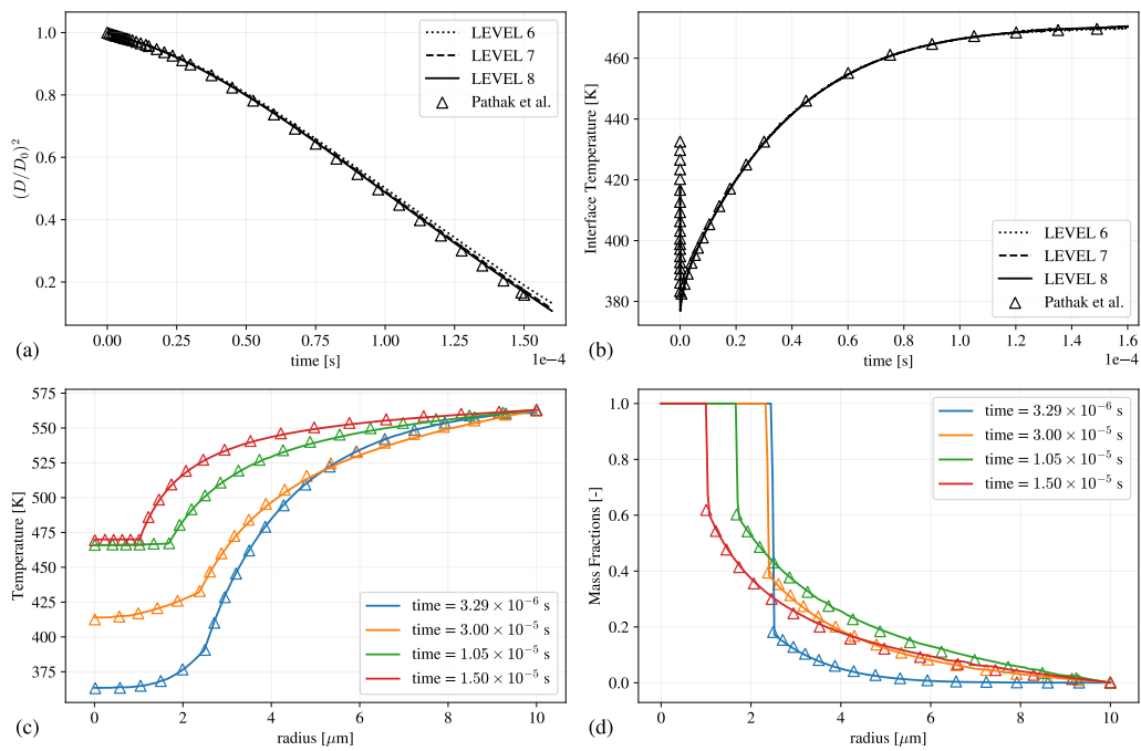
Figure 16: Plots of the square diameter decay in time (a); the interface temperature in time (b); temperature profiles along the domain radius (c); mass fraction profiles along the domain radius (d) ( http://basilisk.fr/sandbox/ecipriano/run/c7pathak.c ).
