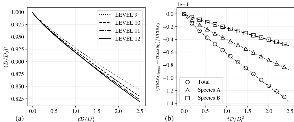
Figure 20: Evolution of the square diameter decay at four different levels of refinement (a); comparison between the variation of liquid mass in the domain for each species (solid line) and the total amount of vaporizing species (markers) normalized by the initial liquid mass (b) at the maximum level of refinement ( http://basilisk.fr/sandbox/ecipriano/run/forcedbi.c ).
