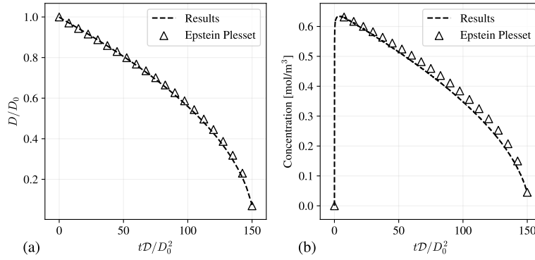
Figure 10: Normalized diameter profile (a), and chemical species concentration at the coordinate R_0+0.2m (b) for the Epstein Plesset problem ( http://basilisk.fr/sandbox/ecipriano/run/epsteinplesset.c ).
