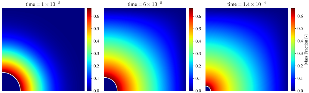
Figure 13: Map of the mass fraction profiles at three different simulation time instants. The white line, representing the interface, is the 0.5 is-contour of the volume fraction field ( http://basilisk.fr/sandbox/ecipriano/run/pureisothermal.c ).
