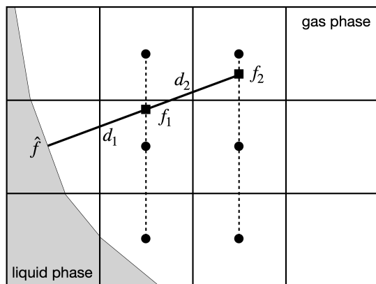
Figure 6: Embedded Boundary Method for the calculation of the interface gradients. Adapted from [36].
