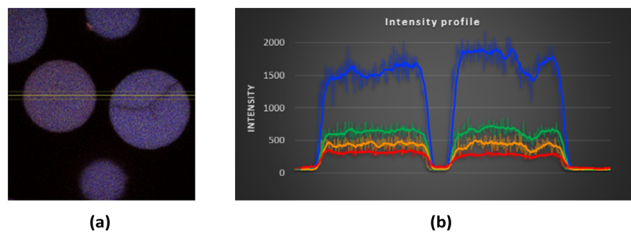
Fig. 3 (a) Image of Tb(DFO)@Purolite resin beads collected under two-photon laser excitation ( \lambda_{\text{ex}} = 750 \text{ nm} ) with an optical fluorescence microscope and (b) terbium-emission intensity profiles collected by the four detection channels along the yellow arrow shown in (a) by moving step-by-step the microscope stage. Blue line: 400–492 nm, green line: 500–550 nm, orange line: 563–588 nm, red line: 601–657 nm.
