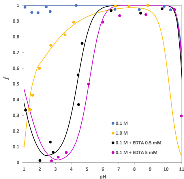
Fig. 10 Sorption profiles of Fe(III) onto DFO@Purolite. Discontinuous procedure: 0.05 g of resin was contacted with 10 mL of 50 \mu M Fe(III) solutions in 0.1 M NaCl (blue dots), 1.0 M NaCl (yellow dots), 0.1 M NaCl containing 0.5 mM Na 2 H 2 EDTA (black dots), and 0.1 M NaCl containing 5 mM Na 2 H 2 EDTA (violet dots). The lines represent the best-fit curves of the experimental data points using eqn (5) and the sorption equilibria given by eqn (13).
