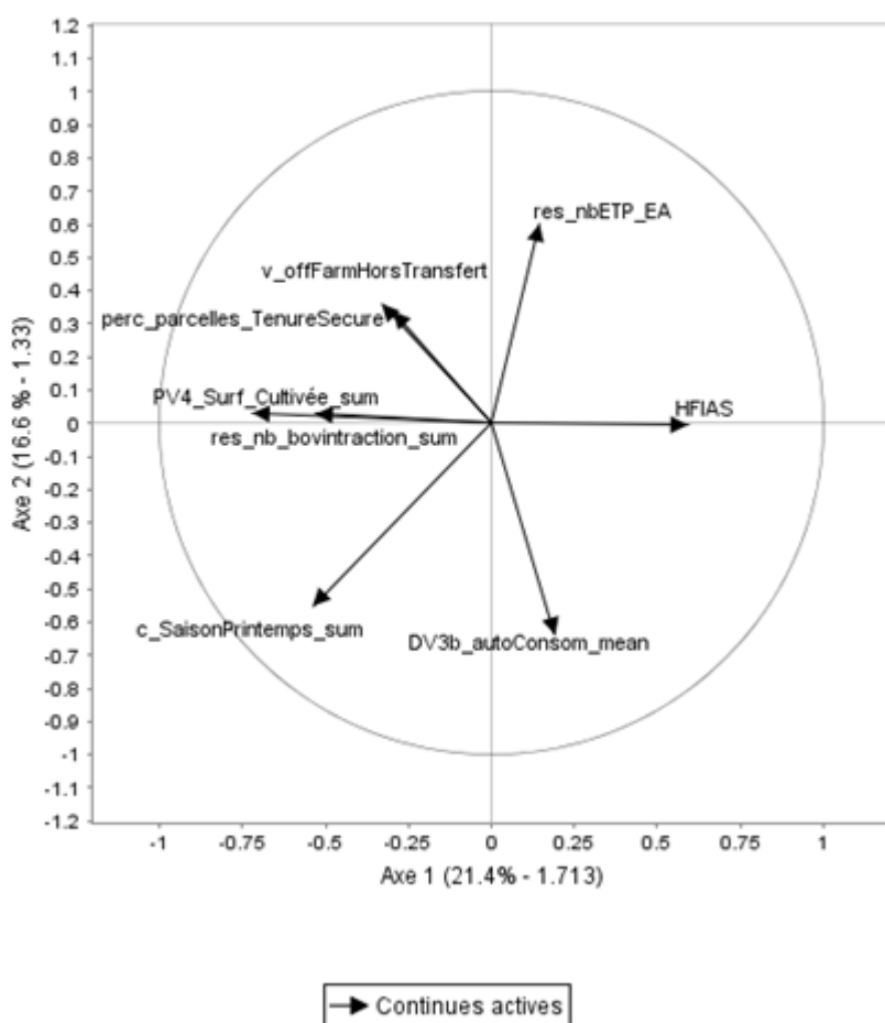
Variables - Axes 1 & 2
