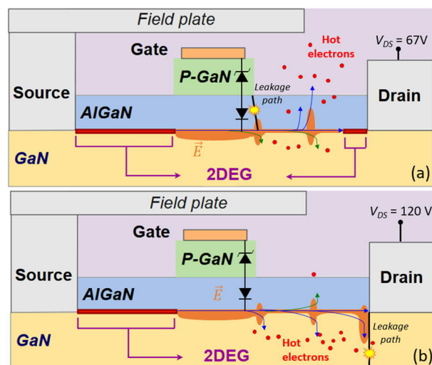
Figure 10: (a) Formation of the gate leakage path through degradation caused by the emission of hot electrons at (a) V_{DS} = 67V and (b) V_{DS} = 120V . The yellow “explosions” symbols illustrate the defect heating/light emission captured with LIT and PEM on Fig. 9 through the GaN layer.
