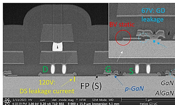
Figure 11: FIB cross-section of the active area showing the location where the defects are expected to be according to our hypothesis. In yellow the drain-source leakage which corresponds to Fig. 4c electrical signature. In blue the gate-drain leakage (Fig. 7ab) which is the failure of D_{pin} diode shown in Fig.10. Also, the form of the metal contact is not perfect due to fabrication maybe thermal relaxation. It makes a small spike and
