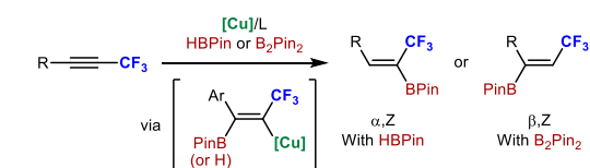
Scheme 1: Hydrometallation of CF_3 -alkynes
