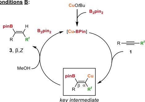
Scheme 4: Proposed mechanisms for the regiodivergent borylation of \text{CF}_3 -alkyne.
