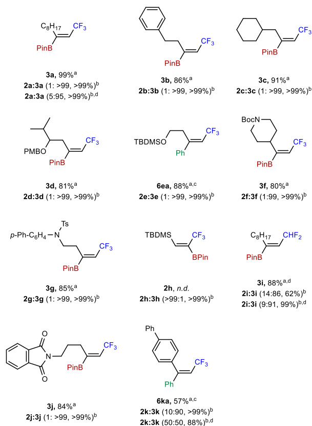
Scheme 3: Regioselective \beta -borylation of R f -alkynes. a Isolated yield. b Ratio 2:3 and NMR yield determined by 19 F and 1 H NMR with PhCF 3 as internal standard. c Obtained after cross-coupling reaction with PhI (1.5 equiv.), Pd(PtBu 3 ) 2 (5 mol%), Cs 2 CO 3 aq. (3 equiv.), 50 °C. d Phox (6 mol%) was used as ligand.
