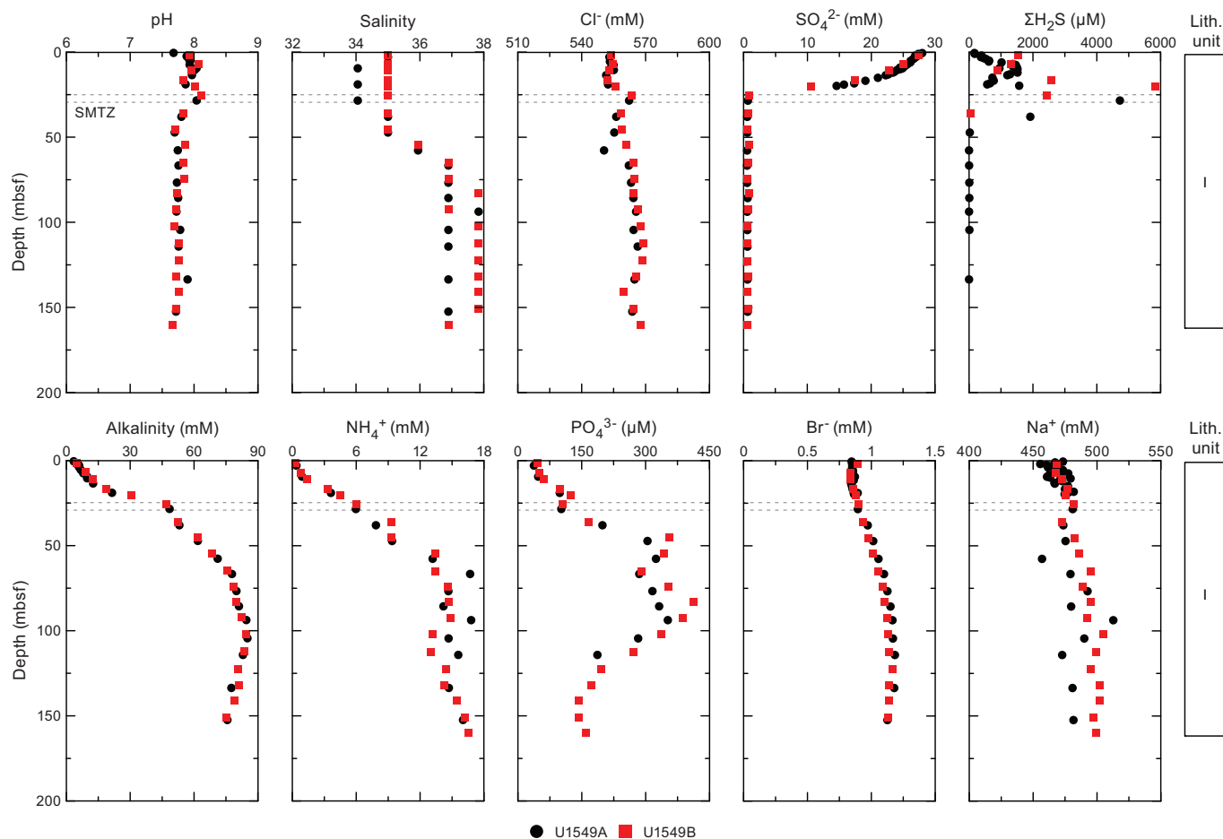
Figure F14. Interstitial water chemistry, Site U1549. SMTZ = sulfate-methane transition zone. (Continued on next page.)
