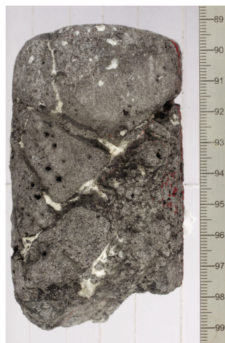
Figure F25. Fault plane displacing small blocks and truncating their bounding fractures in a zone of internal brecciation in hypabyssal igneous rock (385-U1547D-19R-1, 89–100 cm). White vein-filling material (mainly carbonate) is distributed irregularly along the fault and at the intersections with the truncated fractures, indicating that it filled the fractures after slip had taken place on them.
