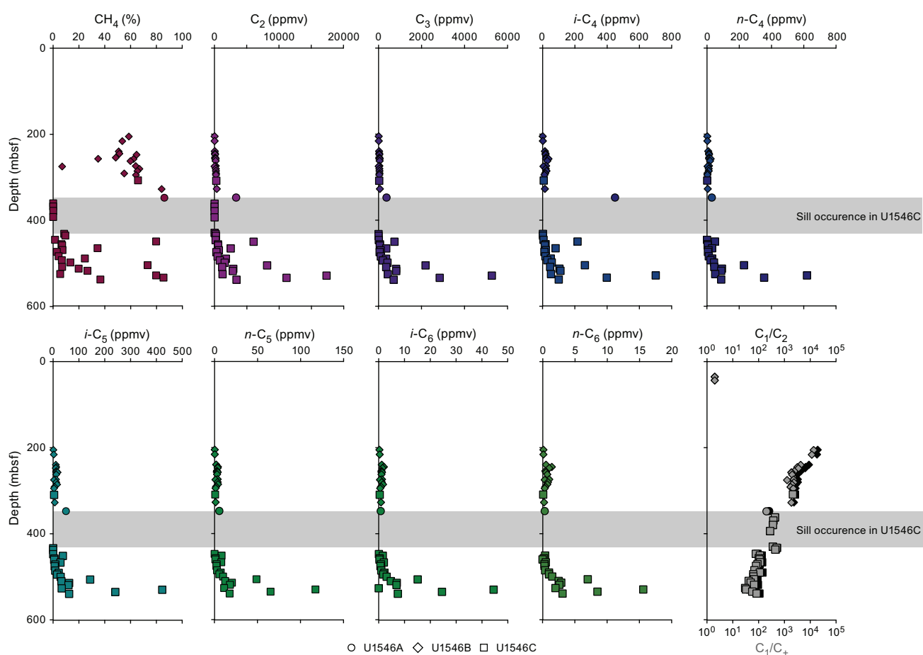
Figure F40. C 1 –C 6 hydrocarbons, C 1 /C 2 , and C 1 /C 4 in void gas samples, Holes U1546A–U1546C.
