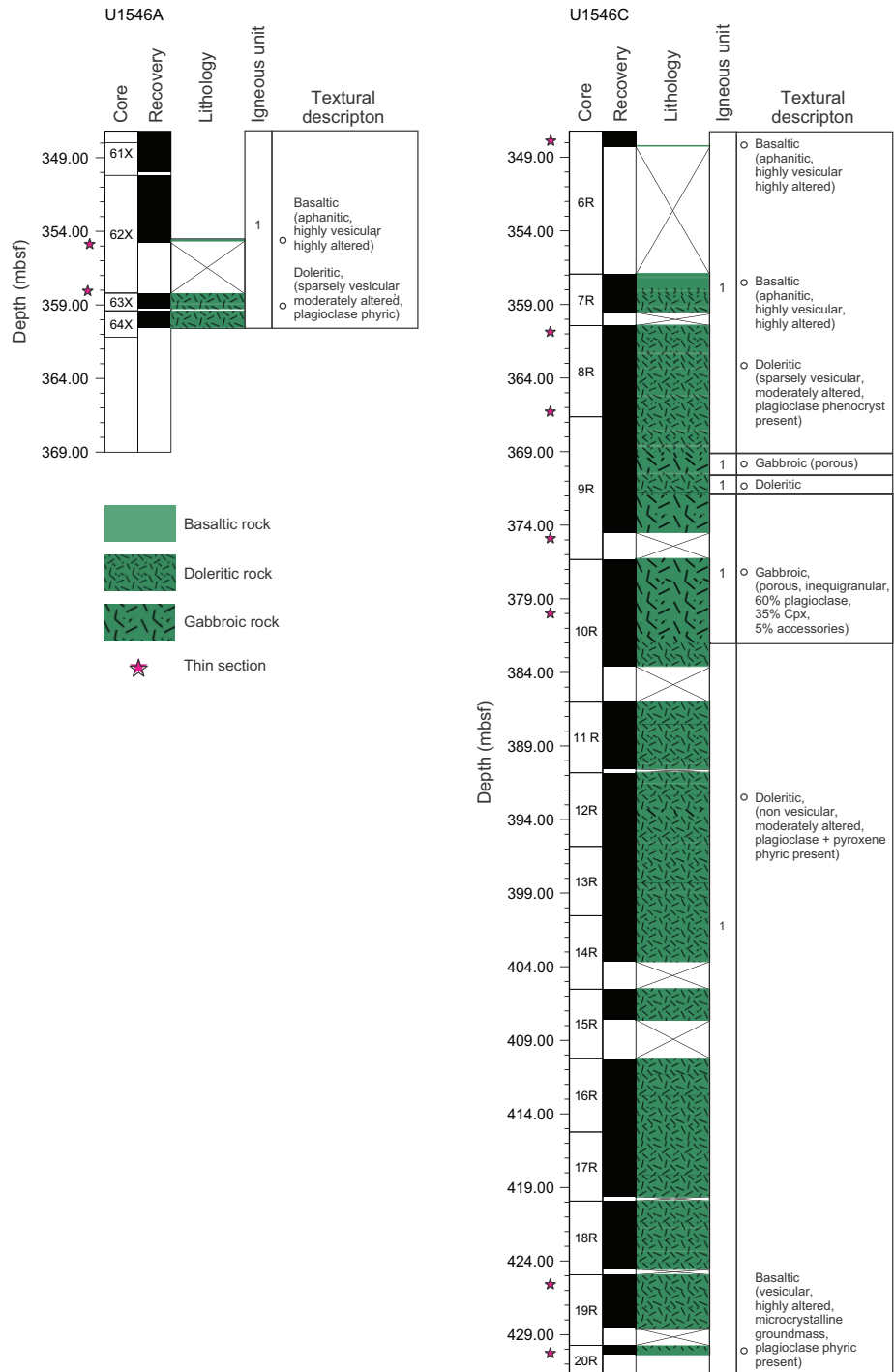
Figure F16. Recovery plots and textural description of the encountered mafic sill, Holes U1546A and U1546C. Cpx = clinopyroxene.
