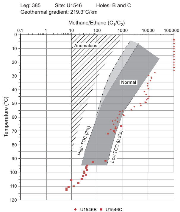
Figure F39. C 1 /C 2 variations in headspace gas with temperature, Holes U1546B and U1546C. TOC = total organic carbon. Modified from Pimmel and Claypool (2001) to include observed extended range of temperature and ratios.
