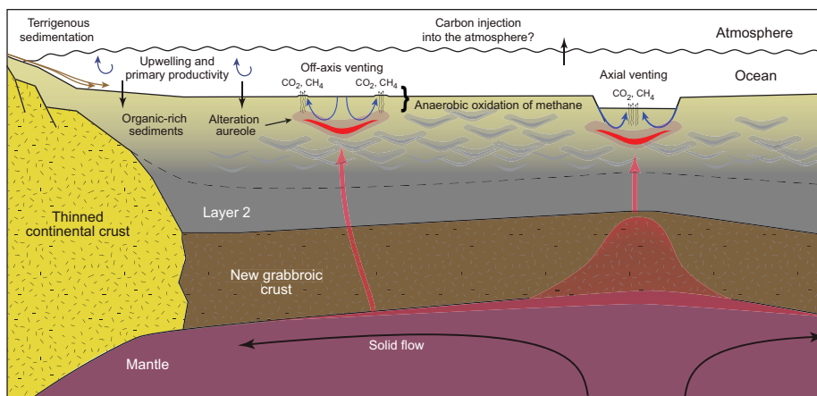
Figure F2. Conceptual model of interacting tectonic, igneous, sedimentological, and microbial processes at work in Guaymas Basin and the associated carbon pathways.
