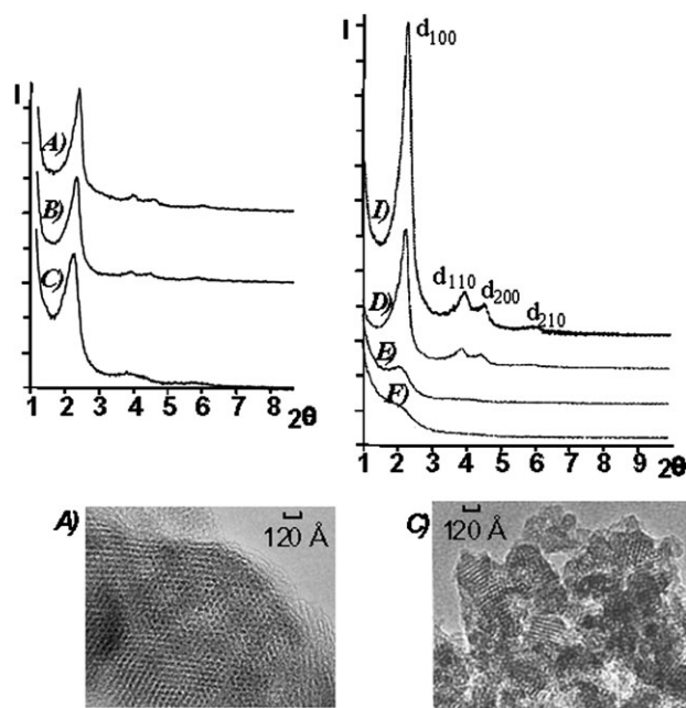
Fig. 2 Upper part: XRD patterns for mesoporous silica containing dendrimers 1-G 4 ( A : Si/ 1-G 4 = 1500; B : Si/ 1-G 4 = 1000; C : Si/ 1-G 4 = 300), 2-Gc 4 ( D : Si/ 2-Gc 4 = 2400; E : Si/ 2-Gc 4 = 750; F : Si/ 2-Gc 4 = 400), and after extraction of CTAB from D ) (I) (molar ratios measured by elemental analyses in all cases). Lower part: TEM images of A ) and C ).
