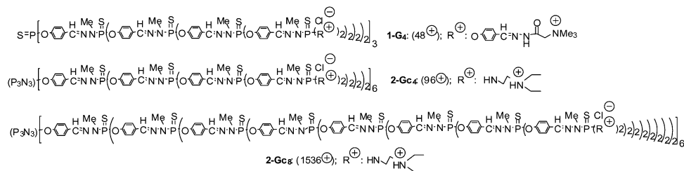
Fig. 1 Chemical structure of the cationic dendrimers used in this study.
