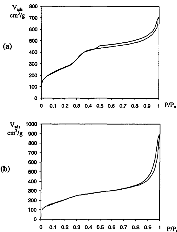
Fig. 4 Isotherms of adsorption and desorption of N 2 (gas) after calcination of the samples A (a) and C (b). Correspondence to liquid adsorbed volume usually used, V_{ads} in cm 3 g -1 will be obtained by multiplying the Y axis values by the factor 0.001547.
