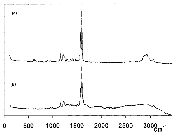
Fig. 7 FT-Raman spectra of sample I (a), and the same sample after reaction with HCl (b).
