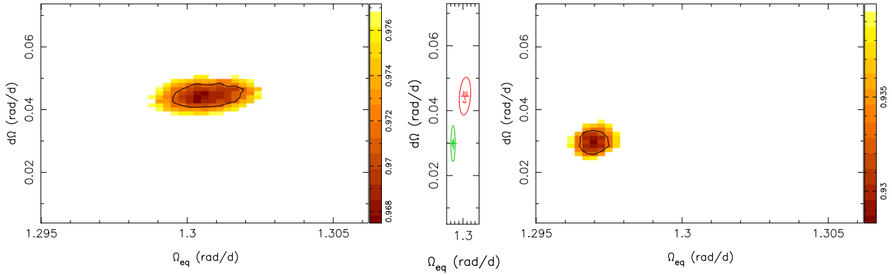
Figure 6. Measuring DR at the surface of AU Mic by minimizing the \chi_r^2 of the ZDI fit to our Stokes V LSD profiles over a grid of DR parameters (see Section 5.4), for season 2020 April–November (left-hand panel) and 2021 June–November (right-hand panel). In both panels, the black contour depicts the 3\sigma confidence interval for the pair of DR parameters. The central panel shows the 1\sigma and 3\sigma confidence ellipses for both seasons (in red for 2020 and green for 2021) together on the same plot.
