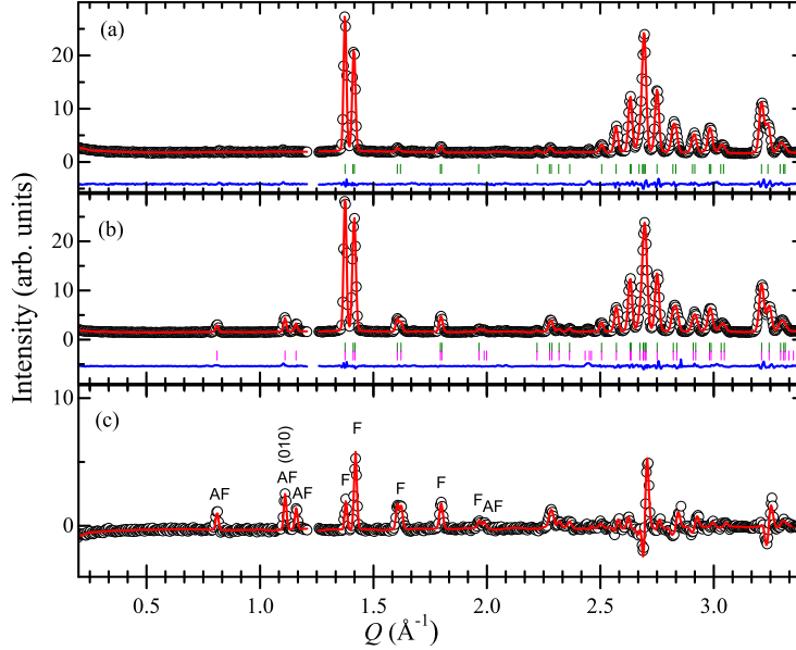
Figure 1. Observed cold neutron powder diffraction profiles of \text{Ca}_{1.7}\text{Y}_{0.3}\text{MnReO}_6 at T = 155 K (a) and T = 3 K (b) (open circles). The difference profile I(3\text{ K}) - I(155\text{ K}) is shown in (c). The calculated profiles for the refined nuclear ( T = 155 K) and nuclear+magnetic ( T = 3 K) structures are shown as red solid lines. The difference curves between observed and calculated profiles are displayed at the bottom of (a) and (b) (blue solid lines). The positions of the symmetry-allowed Bragg reflections are indicated as short green and magenta vertical bars for the nuclear (a and b) and magnetic (b) structures, respectively. In (c), the magnetic reflections arising from ferromagnetic (F) and antiferromagnetic (AF) components are explicitly indicated for Q < 2 \text{ \AA}^{-1} .
