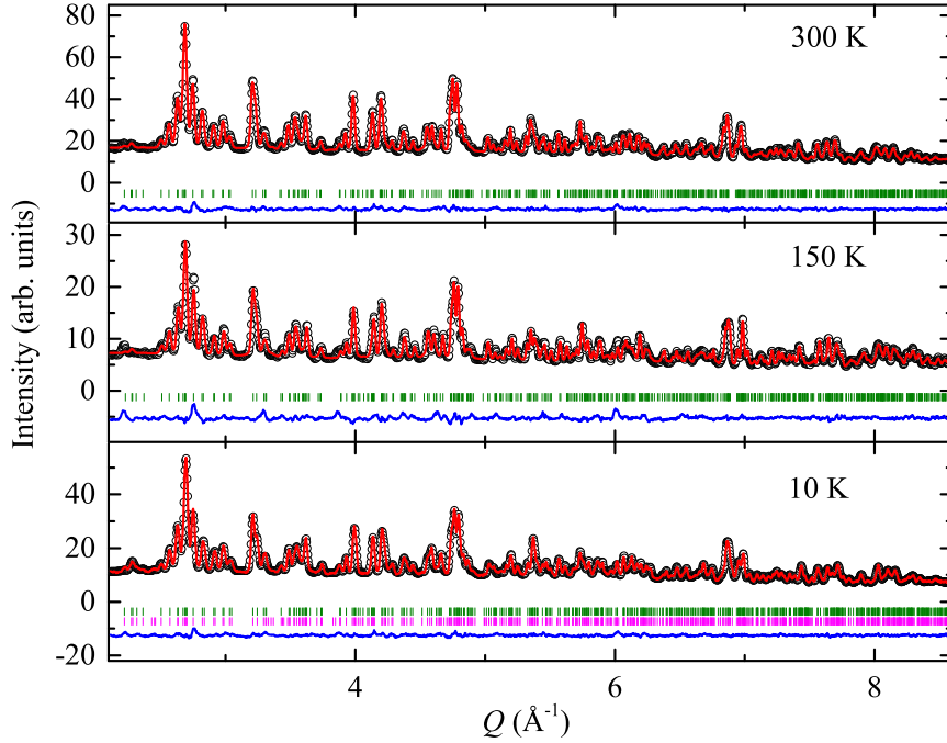
Figure B1. Observed (open symbols) and calculated (red solid lines) thermal neutron powder diffraction profiles of \text{Ca}_{1.7}\text{Y}_{0.3}\text{MnReO}_6 at T = 300 , 150 and 10 K. The difference curves (blue solid line) are displayed at the bottom of each figure. The reflection positions are indicated as short vertical bars for the nuclear structure at all temperatures (green) and for the magnetic structure at T = 10 K (magenta).
