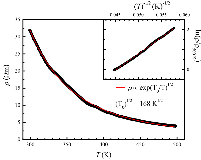
Figure E1. Resistivity as a function of temperature for CYMRO (sample 2) with an exponential fitting (red line) for a \rho \propto \exp(T_0/T)^{1/2} function (ES-VRH model, see text). The inset panel shows the plot of \ln(\rho/\rho_{500K}) versus T^{-1/2} , where \rho_{500K} is the resistivity measured at 500 K.
