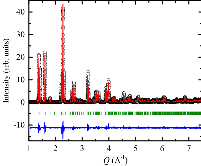
Figure C1. Observed (open symbols) and calculated (red solid lines) X-ray powder diffraction profile of \text{Ca}_{1.7}\text{Y}_{0.3}\text{MnReO}_6 at room temperature. The difference curves (blue solid line) are displayed at the bottom of each figure. The reflection positions are indicated in short vertical bars.
