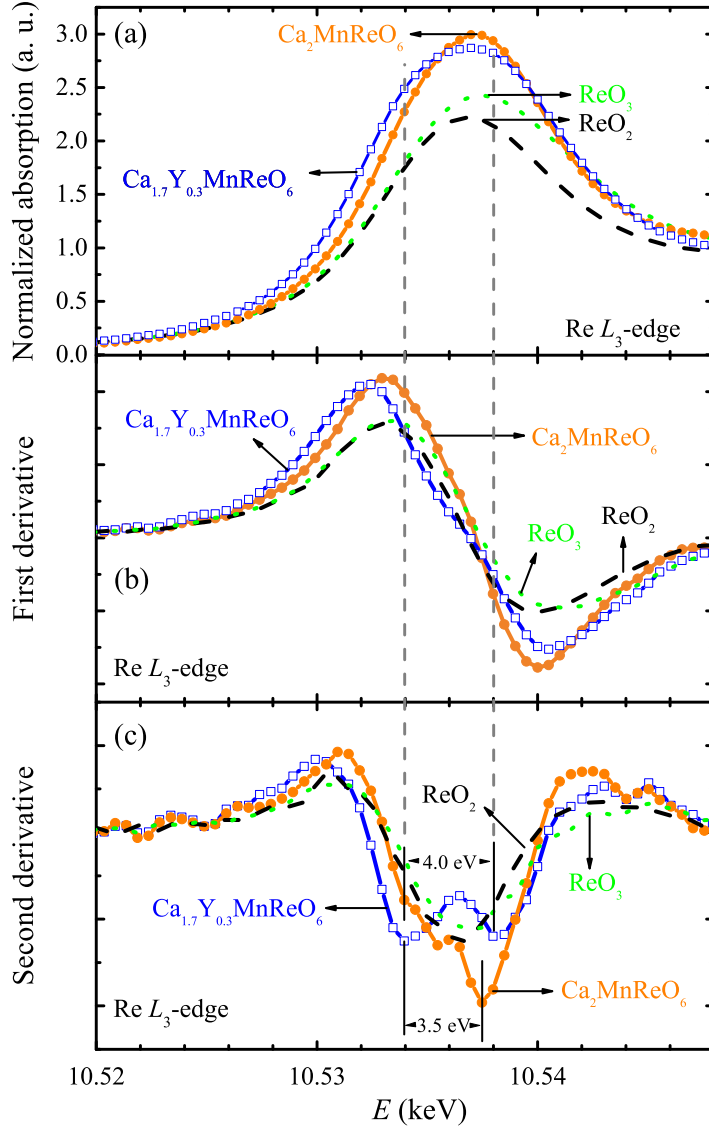
Figure 6. (a) Re L_3 XANES of CMRO, CYMRO (symbols), and the reference materials ReO_2 (dashed line) and ReO_3 (dotted line). (b) First and (c) second derivatives XANES spectrum of CMRO and CYMRO at the Re L_3 edge.
