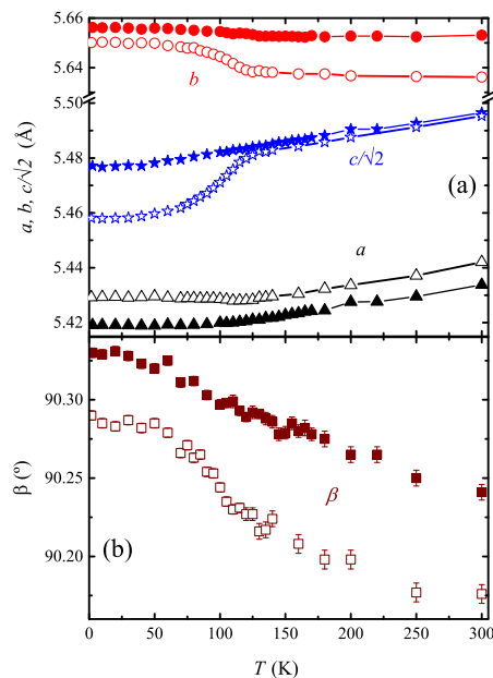
Figure 2. Temperature dependence of the (a) lattice parameters and (b) \beta angle of \text{Ca}_{1.7}\text{Y}_{0.3}\text{MnReO}_6 (filled symbols) in comparison to the parent compound \text{Ca}_2\text{MnReO}_6 (open symbols, taken from Reference [3]). The statistical errors in (a) are not displayed for being smaller than the symbol size.
